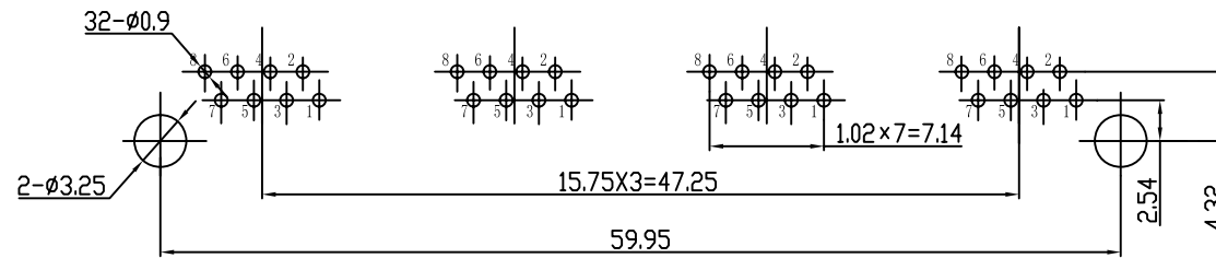
PC Board Layout
